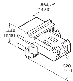
Two-Position Only 641533-1
