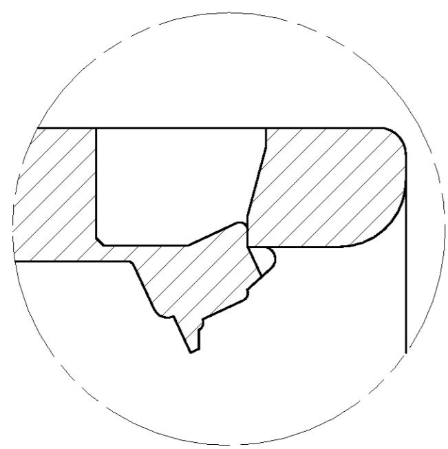
⑤ DETAIL A LATCH POSITION AFTER CRIMPING SCALE 10:1
