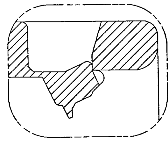
DETAIL A (5) SCALE 10:1
