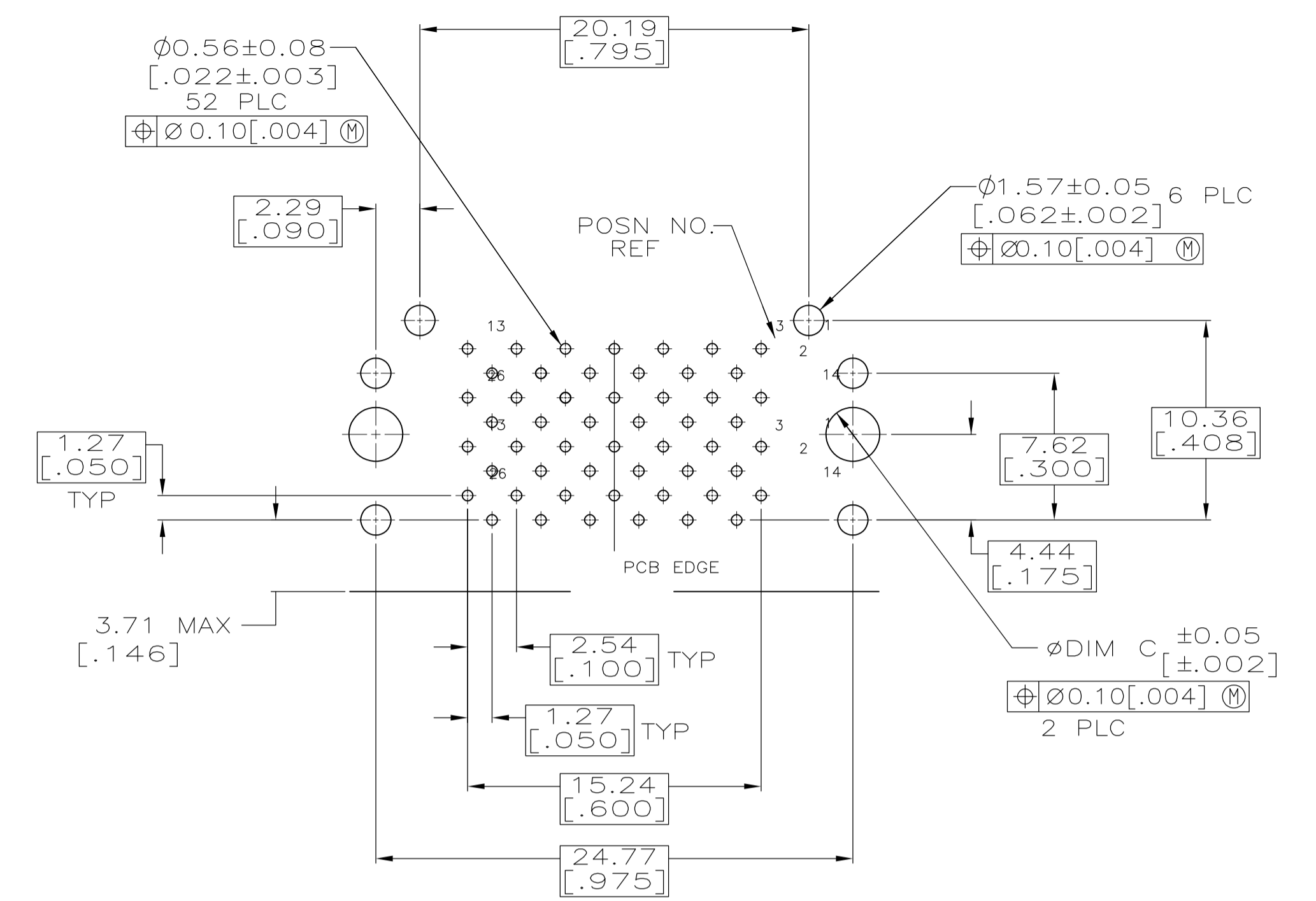
P.C. BOARD MOUNTING DIMENSIONS CONNECTOR SIDE PC BOARD THICKNESS = DIM D [±0.08]
