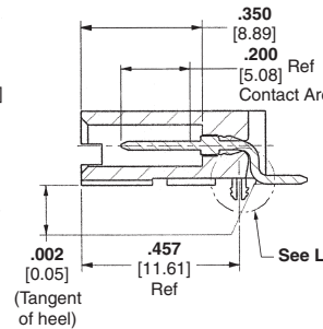
Section K-K
