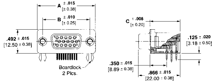
Right-Angle Receptacle
