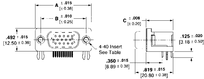
Right-Angle Plug
