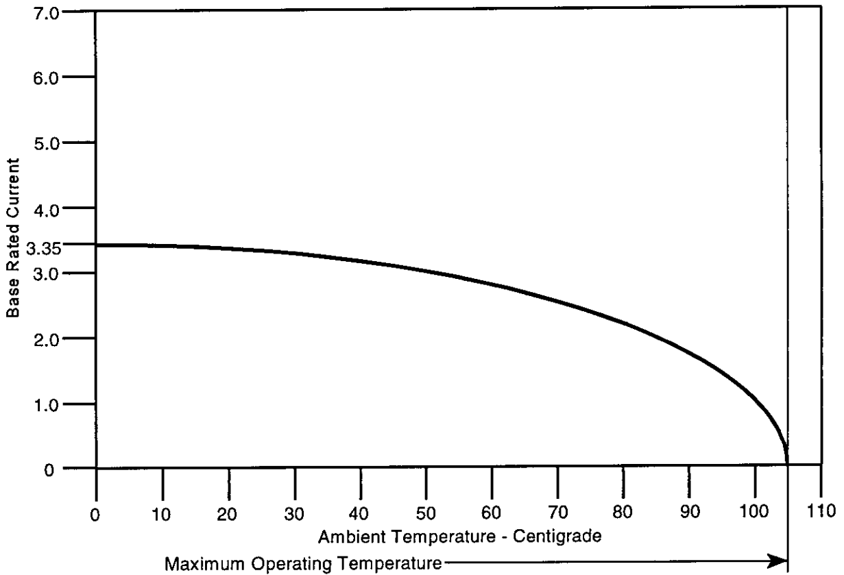
Figure 5A Current Carrying Capability
