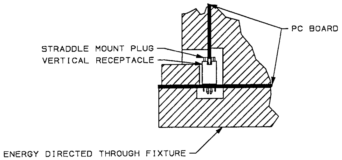
Figure 6 Vibration & Physical Shock Mounting Fixtures
