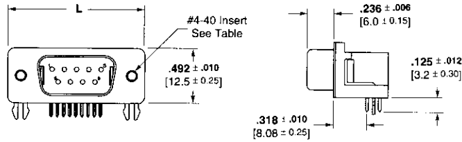
Typical Plug
