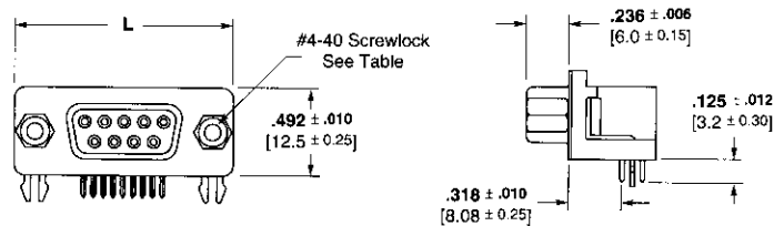
Typical Receptacle
