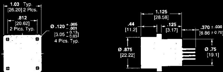
Part Number 447914-1
