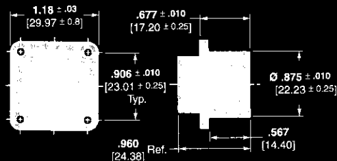
Part Number 864900-1 (Supplied with Contacts)
