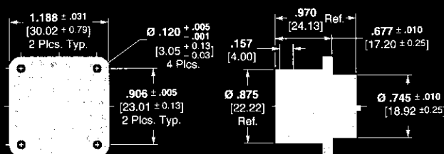
Part Number 864900-1 (Supplied with Contacts)
