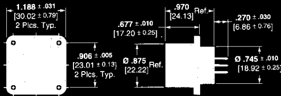
Part Number 447913-1
