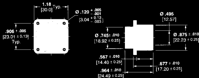
Part Number 449652-1
