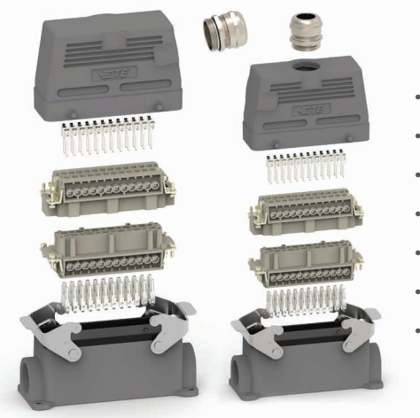
(III) Side entry (IV) Top entry
