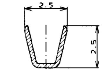
断面 "A"- "A" SECT.
