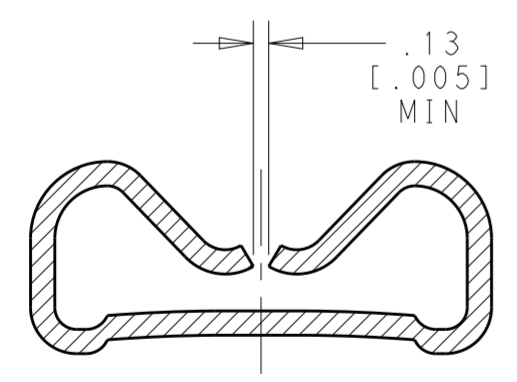
SECTION X-X SCALE 8:1
