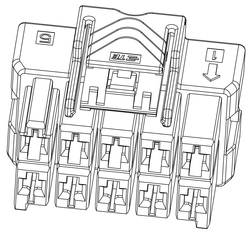
2*5 POSITIONS
