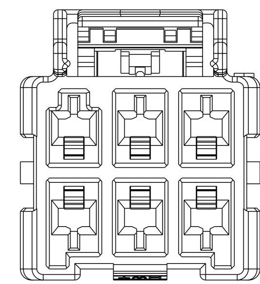
2*3 POSITIONS
