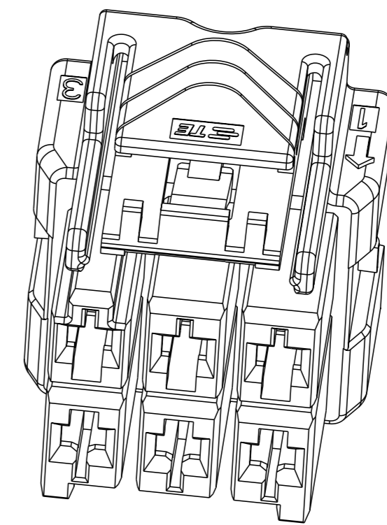
2*3 POSITIONS
