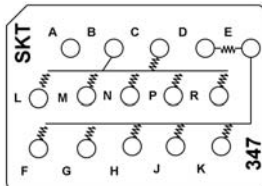
CTJ420E347 Twelve 4.99 k \Omega Resistors, 1/8 W
