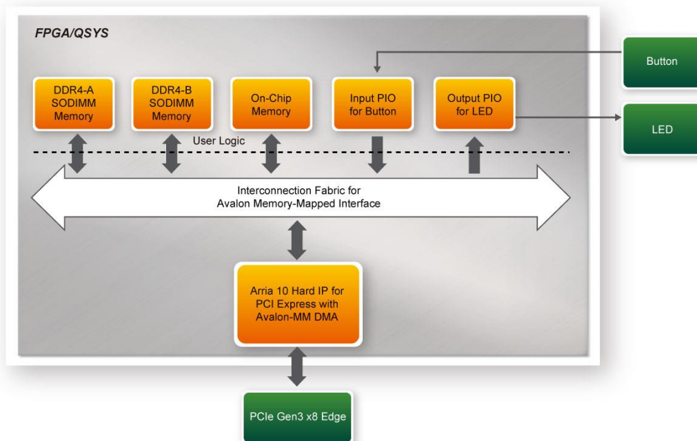
Figure 8-16 Hardware block diagram of the PCIe_DDR4 reference design
