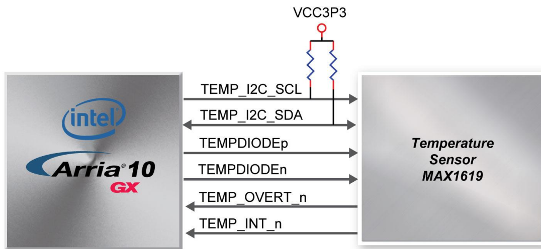
Figure 2-9 Connections between the temperature sensor and FPGA
