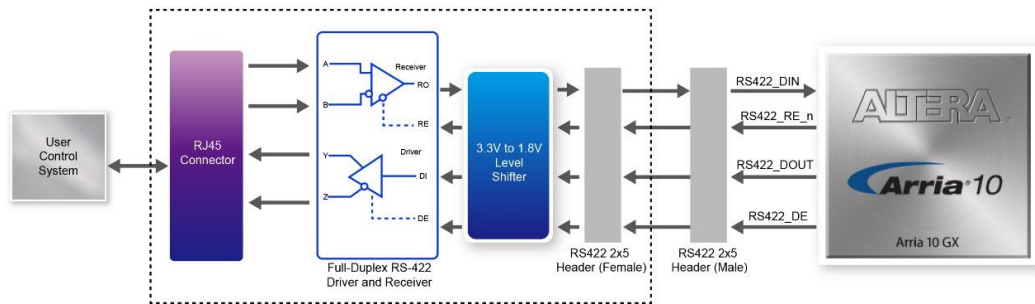
Figure 2-17 Block Diagram of RS-422 application
