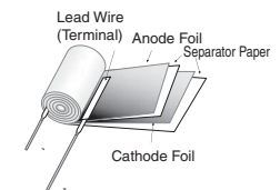
Winding Model
