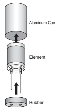
Sealing Model
