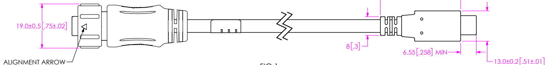
FIG 1 BCU-C-X-X.XX-UC-P SHOWN
