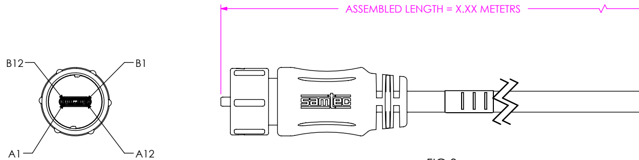
FIG 3 BCU-C-X-X.XX-BC-P SHOWN (DIFFERENT AS SHOWN, OTHERWISE SAME AS FIG 1)
