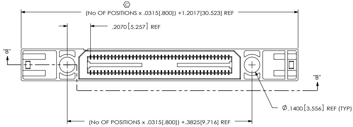
FIG 2 -GP: GUIDE POST BSE-040-01-X-D-EM2-GP SHOWN (60 POSITION MAX) [DIFFERENT AS SHOWN, OTHERWISE SAME AS FIG 1]
