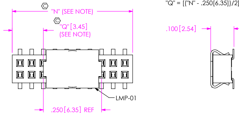
FIG 3 -P: PICK AND PLACE PAD (NOT AVAILABLE WITH -PA OR -K OPTIONS)
