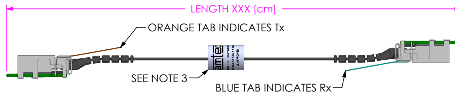
PART NUMBER ETUO-U12-XX-XXX-0-1-1-5 SHOWN
