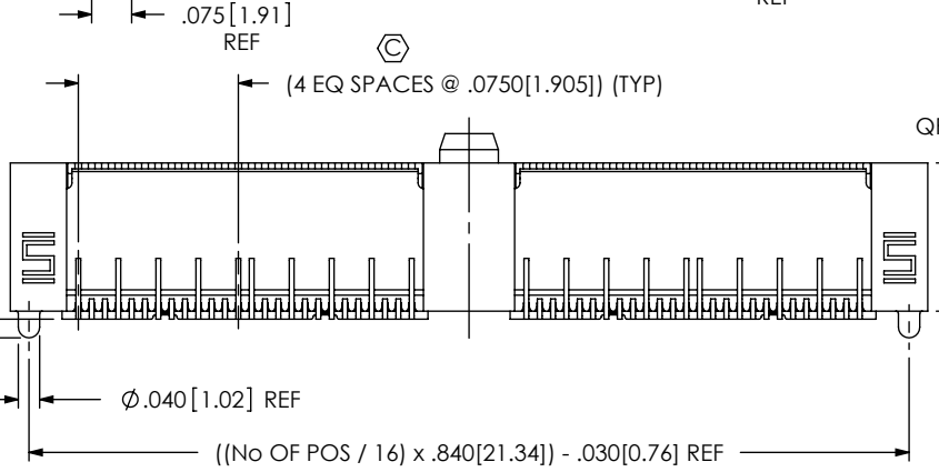
FIG 1 QFSS-032-04.25-X-D-DP-A SHOWN
