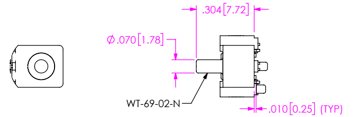
FIG 5 -PP OPTION (SE AFC-20-05.0-XX-06-1-A-PP-K-TR SHOWN) (SOME CENTER FEATURES REMOVED FOR CLARITY) (SAME AS FIG 5 EXCEPT AS SHOWN) (-PP OPTION VALID FOR SEAR MATE ONLY) (ONLY AVAILABLE WITH -.05.0 LEAD STYLE 6, 8 & 10 ROW)
