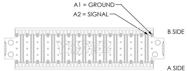
PCB 1 SHOWN
