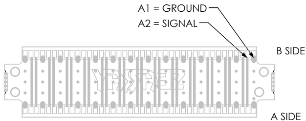
PCB 1 SHOWN
