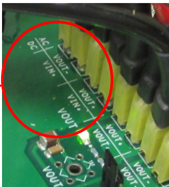
Figure 6 - Power Connections
