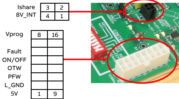
Figure 8 - Signal connector
