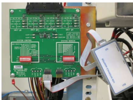
Figure 16 - The latest CPL Interface Module and USB Interface Adapter
