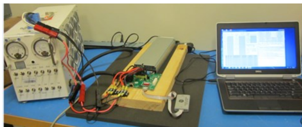
Figure 1 - Single module test setup using the Single Module CPL interface card
