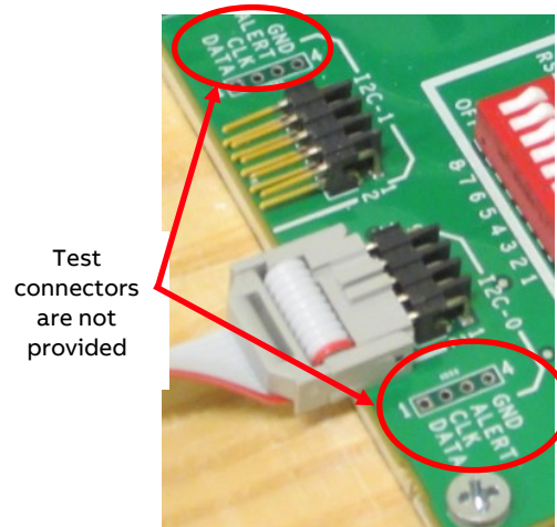
Figure 5 - Signal Connections
