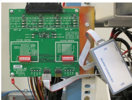
Figure 12 - CPL Shelf module connected to the ABB Adapter
