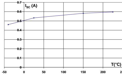
Figure 3: Short-circuit current vs. T^\circ
