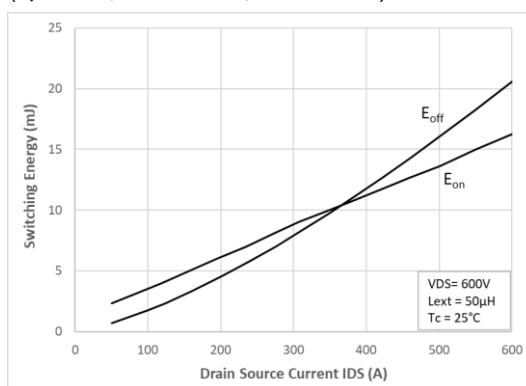
Figure 10 : Switching Energy
