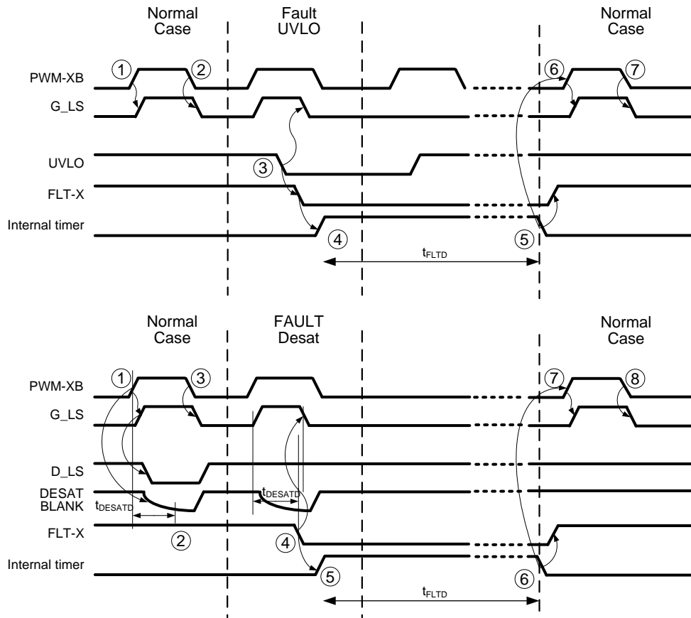
Figure 26: Timing diagram CXT-PLA3SA12550A low-side gate driver behaviour
