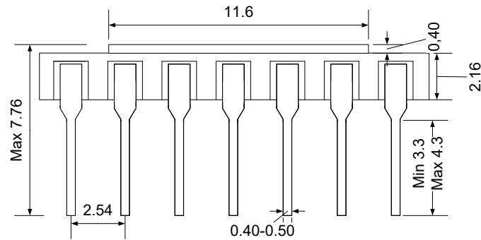
Drawing CDIL14 (mm +/- 10%)
