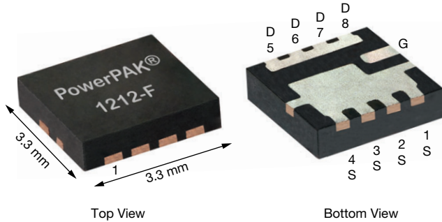
PowerPAK® 1212-F
