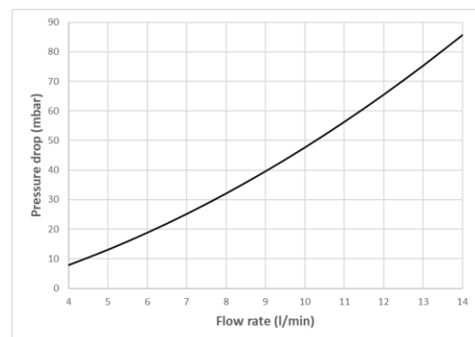
Figure 25: Pressure drop in cooling circuit
