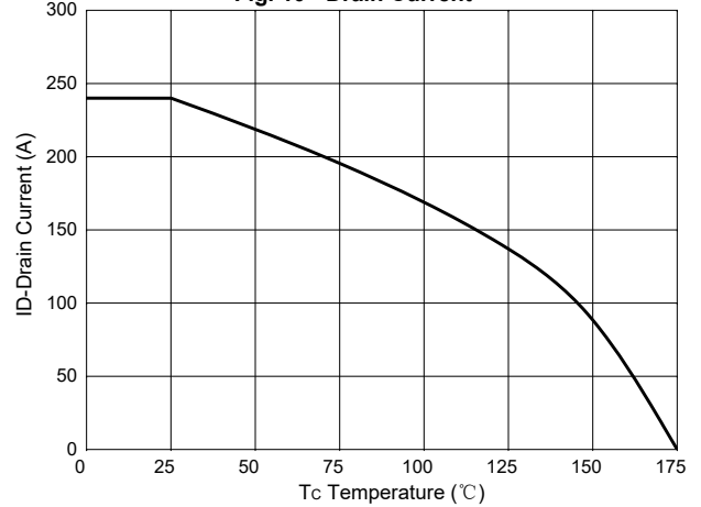
Fig. 10 - Drain Current
